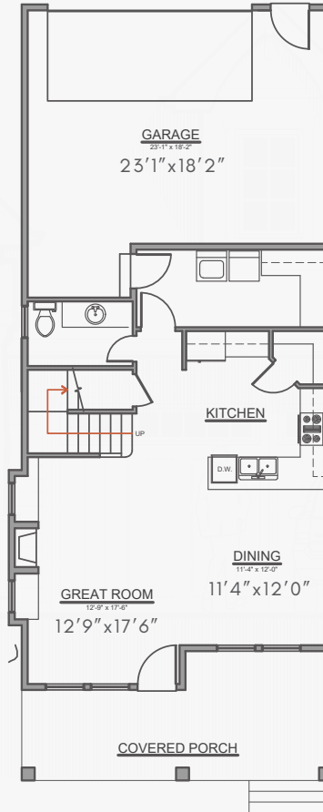
LOWER FLOOR PLAN
