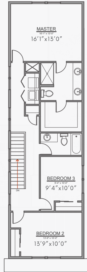
UPPER FLOOR PLAN
